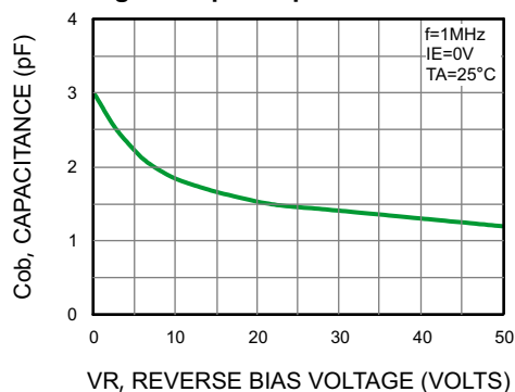
Fig 4. Output Capacitance
