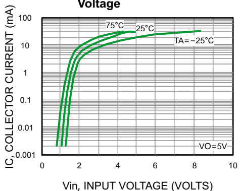
Figure 5. Input Voltage versus Output Current
